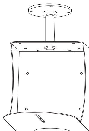
Pole Mount
